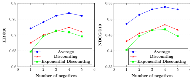
Figure 4: Performance of our model w.r.t number of negative samples
